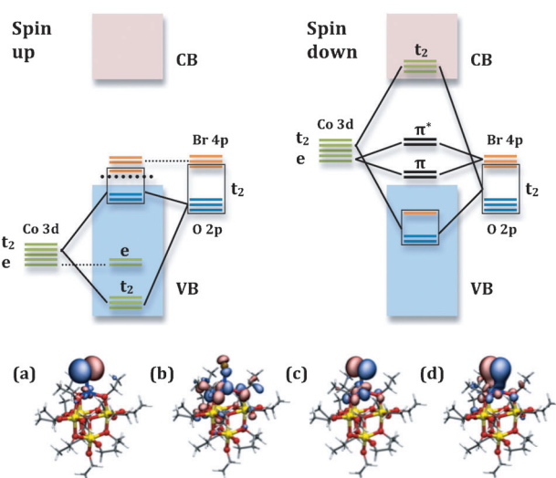
Figure 3. Orbital interaction diagram of cage 1 based on B3LYP calculations. The molecular orbitals of the band-gap states are shown in (a)–(d); a) and b) correspond to states i and iii in the spin-up channel, and c) and d) are states iv and v in the spin-down channel. See text for details.
